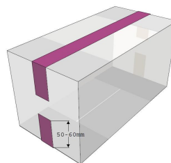
Überlappung ca. 50-60mm Fig. 1
